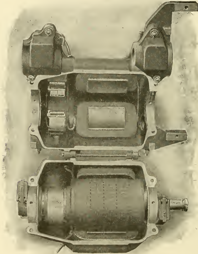
Fig. 32. Westinghouse Railway Motor—Lower Field Down
